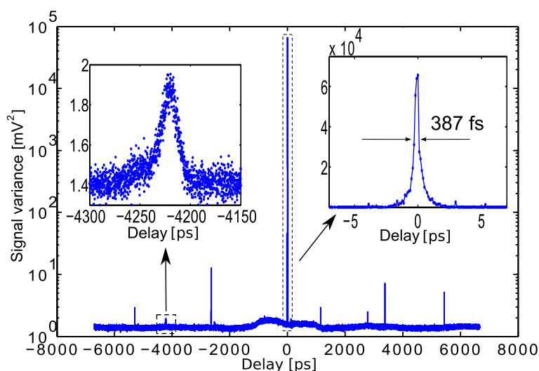
Fig. 4. Semi-logarithmic plot of the variance of the interferometric signal resulting from the averaging of 1.5 \times 10^9 laser shots. The right insert shows a zoom of the main peak evidencing the time resolution (linear scale). The left insert shows a small feature observed 4 ns away from the main peak (linear scale).
