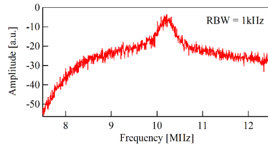
図 7 f_{CEObeat} (log scale)
