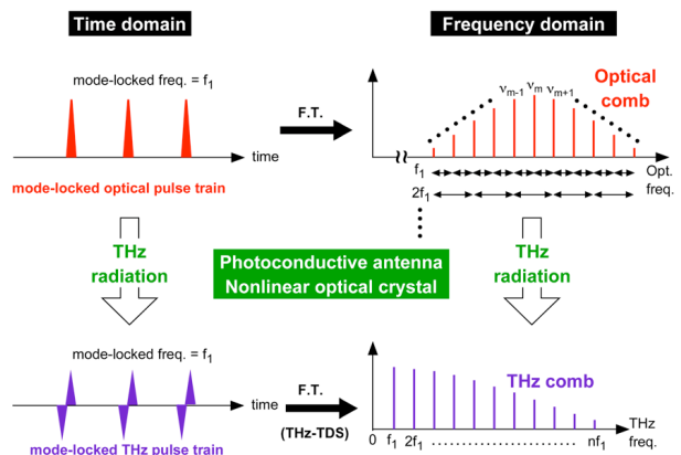
Fig. 1 Optical frequency comb and THz comb
