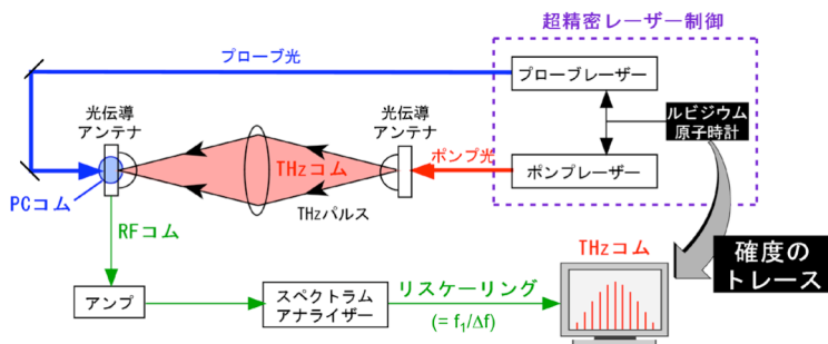
Fig. 2 Experimental setup
