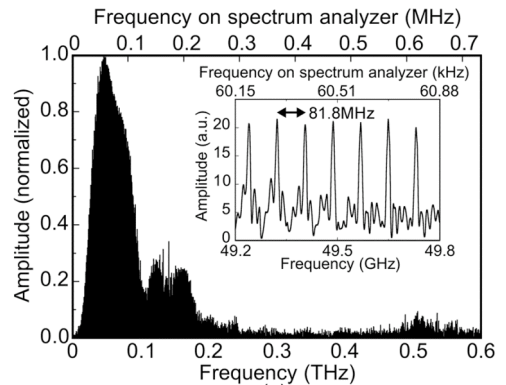
Fig. 4 Amplitude spectrum of THz comb
